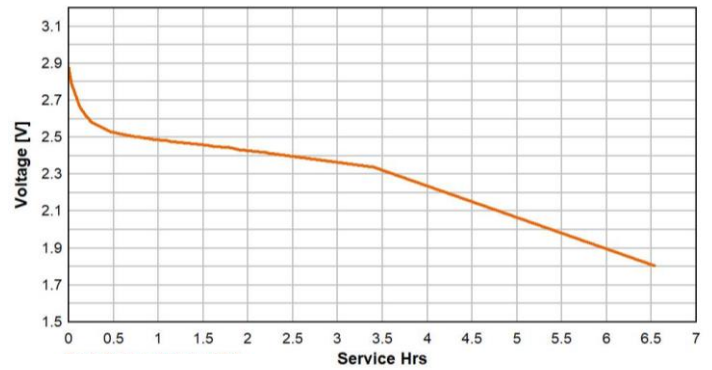
High Resistance Test 65Ω/12mA to 1.8V
