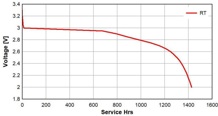
Temperature Discharge Characteristics 15k Ω Cont. to 2V
