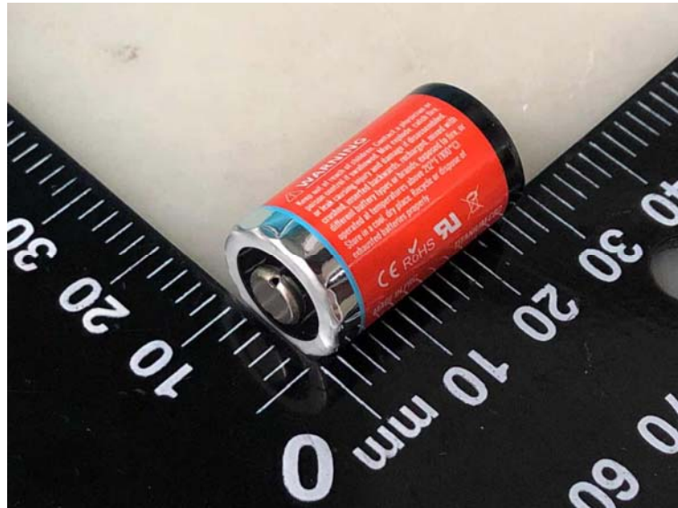
Cell/电芯 (CR2(CR15270) 3,0V 1000mAh)
